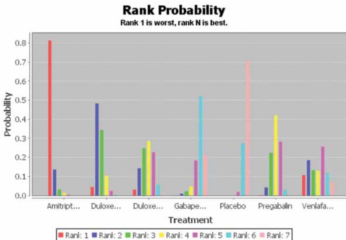
Fig 3. Ranking probabilities for each drug based on the safety.
